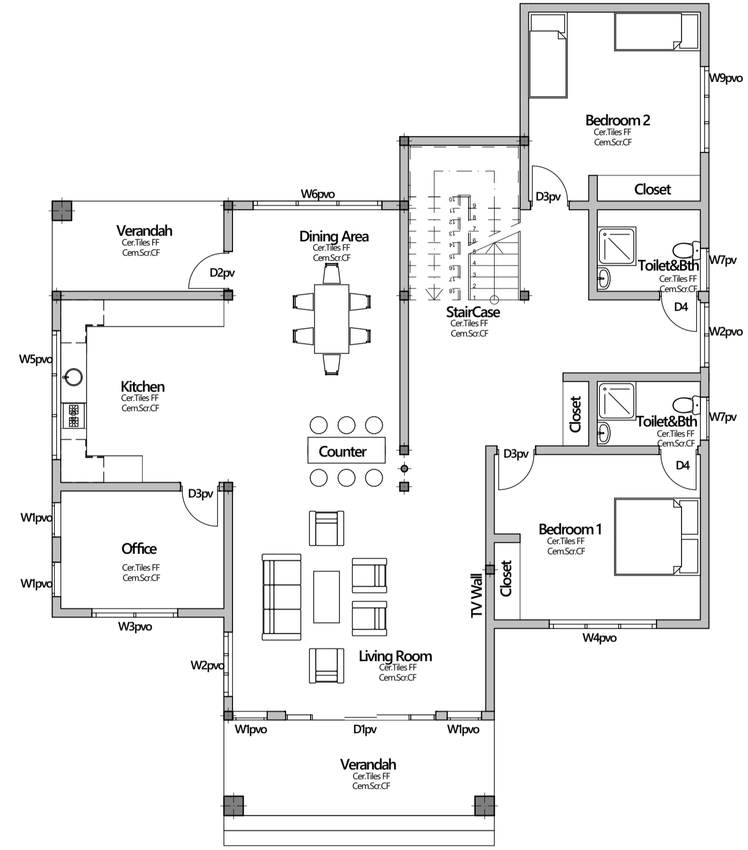
0. Ground Floor Plan 1:90
